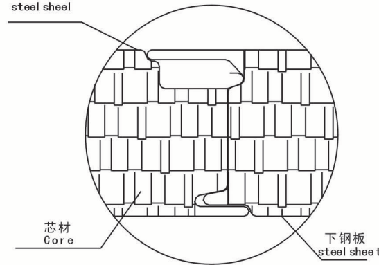
隐藏式墙面板接口 The cryptic undee wall panel joint
