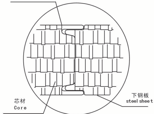
插接式墙面板接口 The jack wall panel joint
