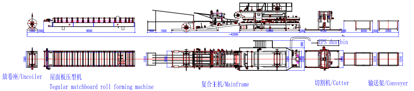
PRL-5C设备排布图/The sketch of PRL-5C
